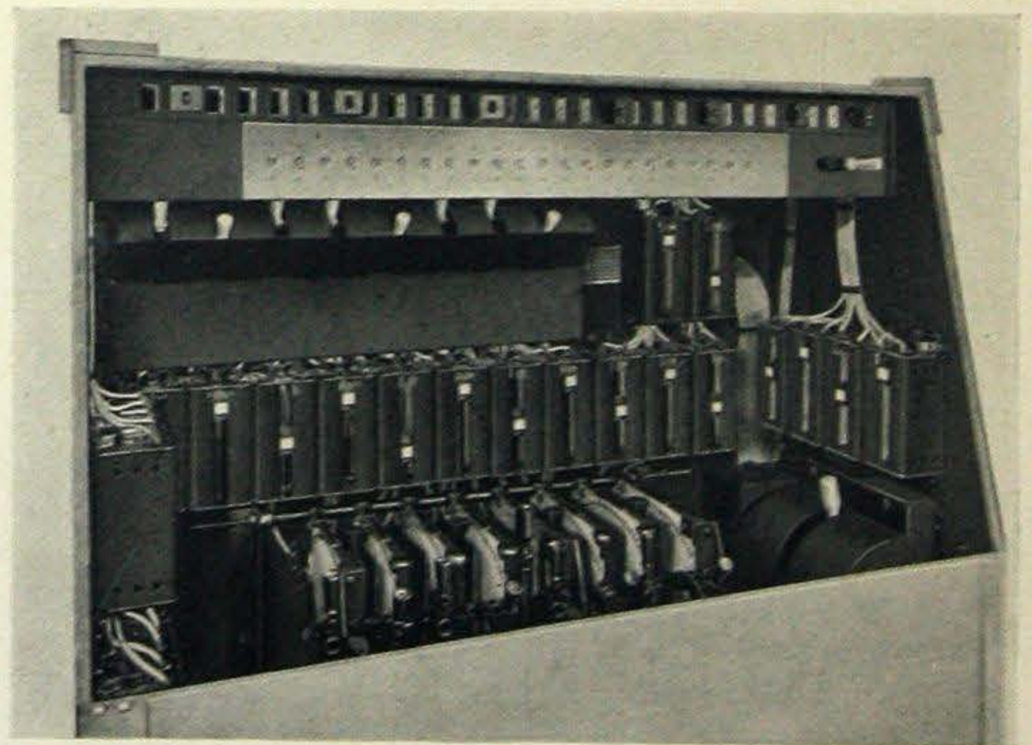
400-ampere Portable Dimmer equipment manufactured by the New York Calcium Light Company, using 8 standard rectangular Vitrohm plates and 18 slide type Vitrohm spotlight dimmers.
