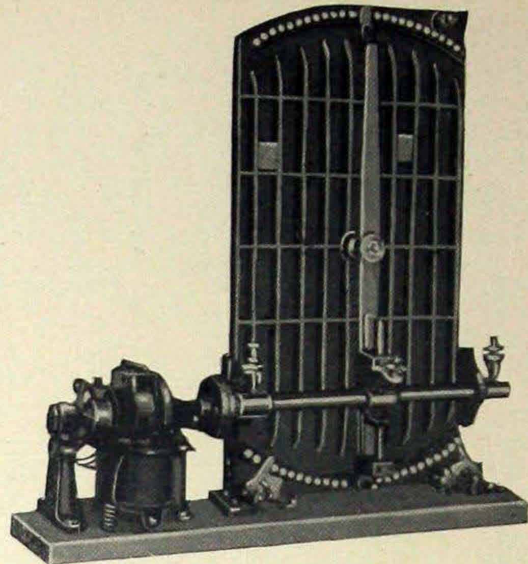
Figure 31—Ward Leonard remote control dimmer operated by three push buttons—1897. This dimmer is still used in the Waldorf-Astoria auditorium.
