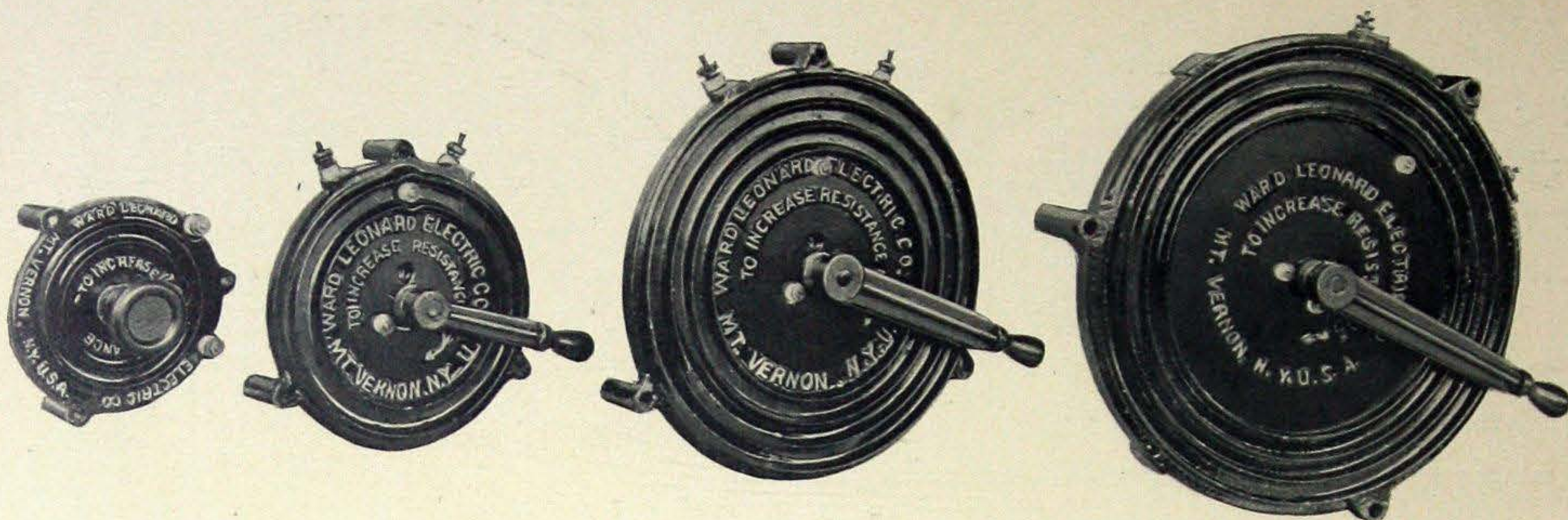
Figure 43—Variety of sizes of Ward Leonard dimmer rheostats for single-plate installations.
