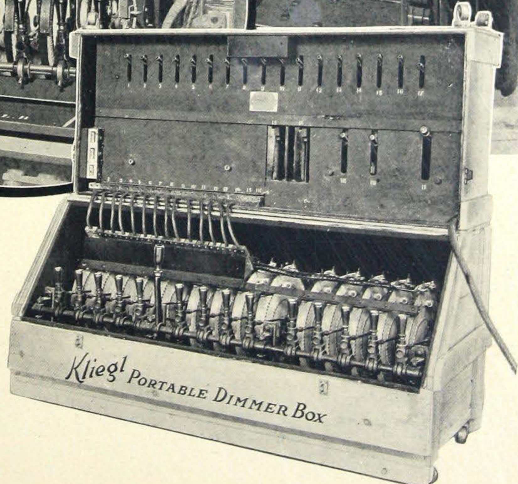
Portable Dimmer equipment made by Kliegl Bros., New York, using Vitrohm round plates.
