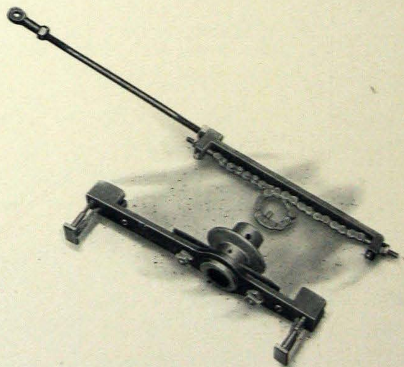
Figure 40—Contact arm and contact-arm drive of Ward Leonard Vitrohm dimmer plate. The contact shoes are provided with long plungers which permit them to ride easily over the contacts and maintain a proper contact pressure under all conditions. The drive gives a positive, though flexible connection that operates with little friction.
