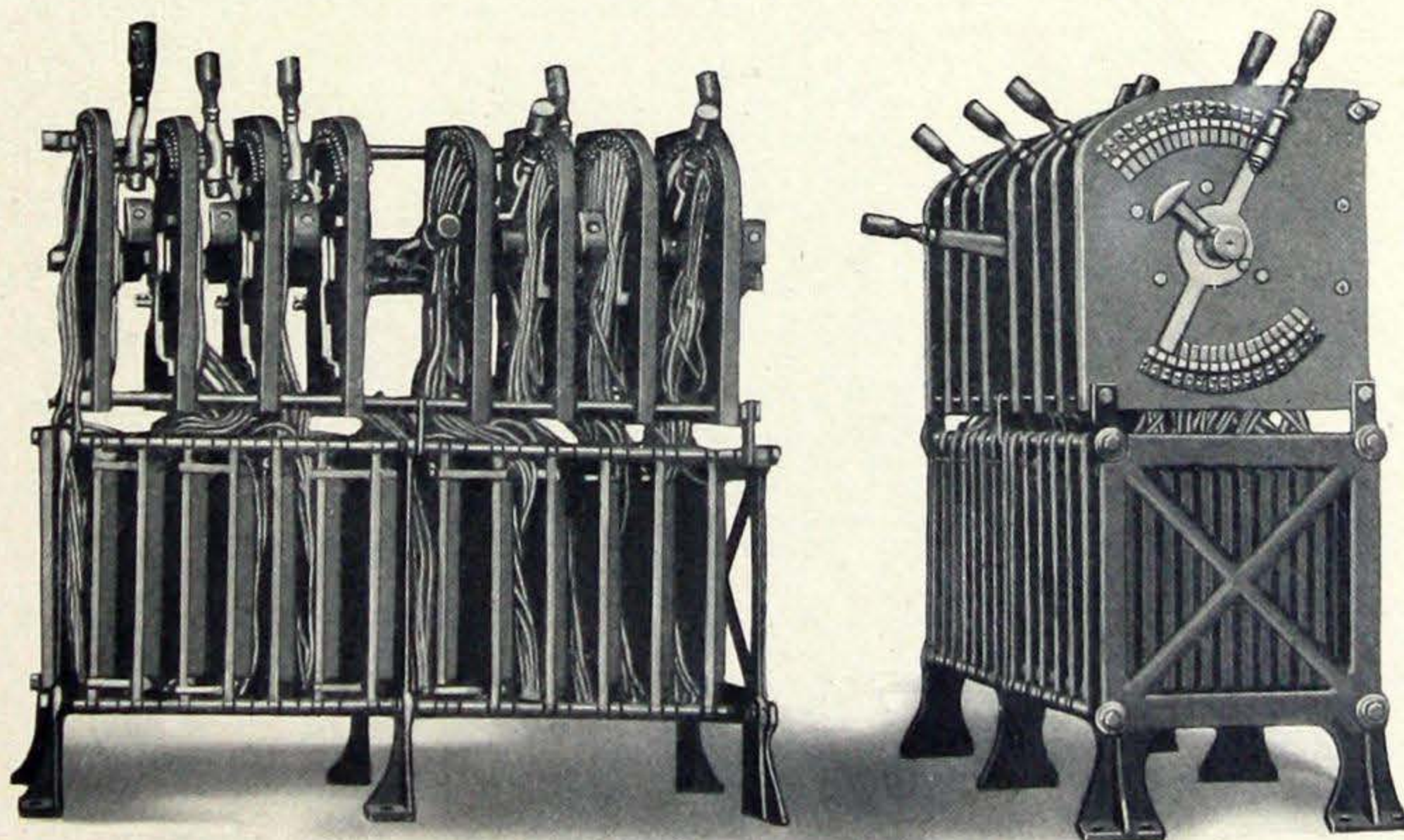
Figure 26—Ward Leonard Theatre Dimmer put on the market in 1894. It consisted of banks of vitrohms rectangular plates mounted in a frame work above which dial switches were arranged. Connections between the contact points on the dial switch and corresponding points in the resistor units were made by means of wires. This was the first step in decreasing the space occupied by a bank of theatre dimmers.
