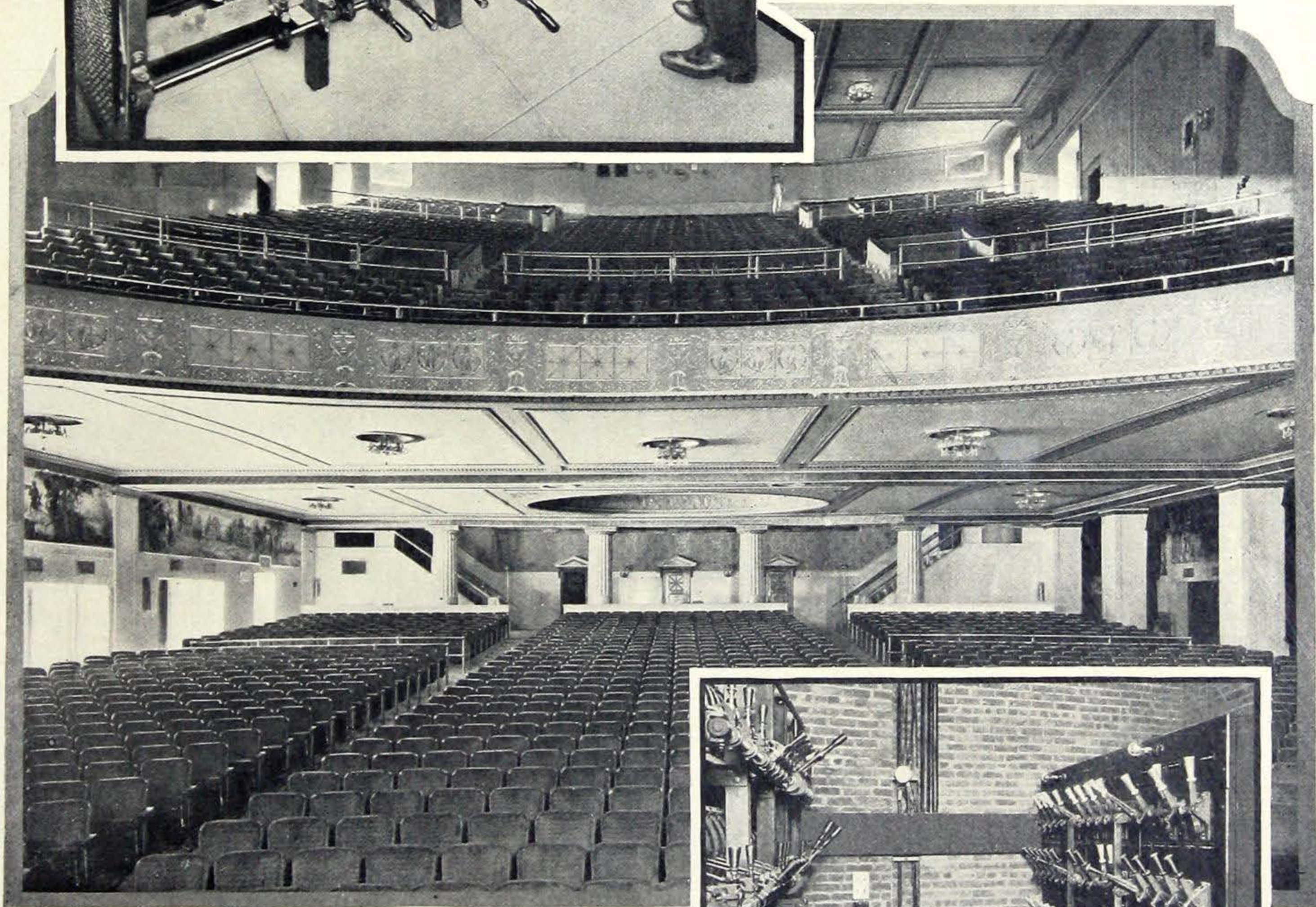
Ward Leonard Dimmer Bank installed in the State Theatre in Jersey City, N. J. This dimmer regulates the colored lights in the elaborate chandelier above the auditorium, as well as the stage lighting.
