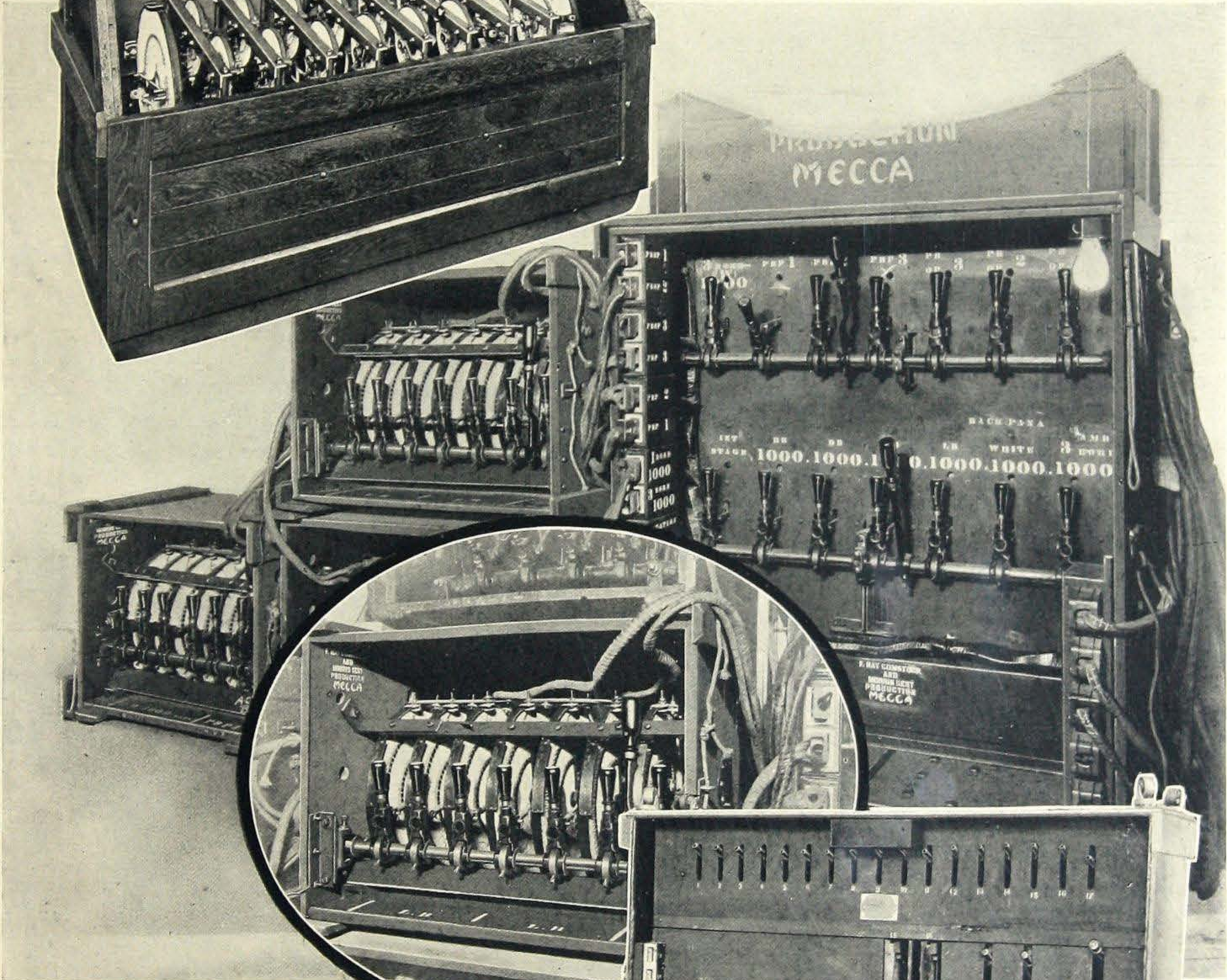
Portable Dimmer equipment made especially for the spectacular show, "Mecca," using Vitrohm round plates and Ward Leonard control levers on the switchboard.
